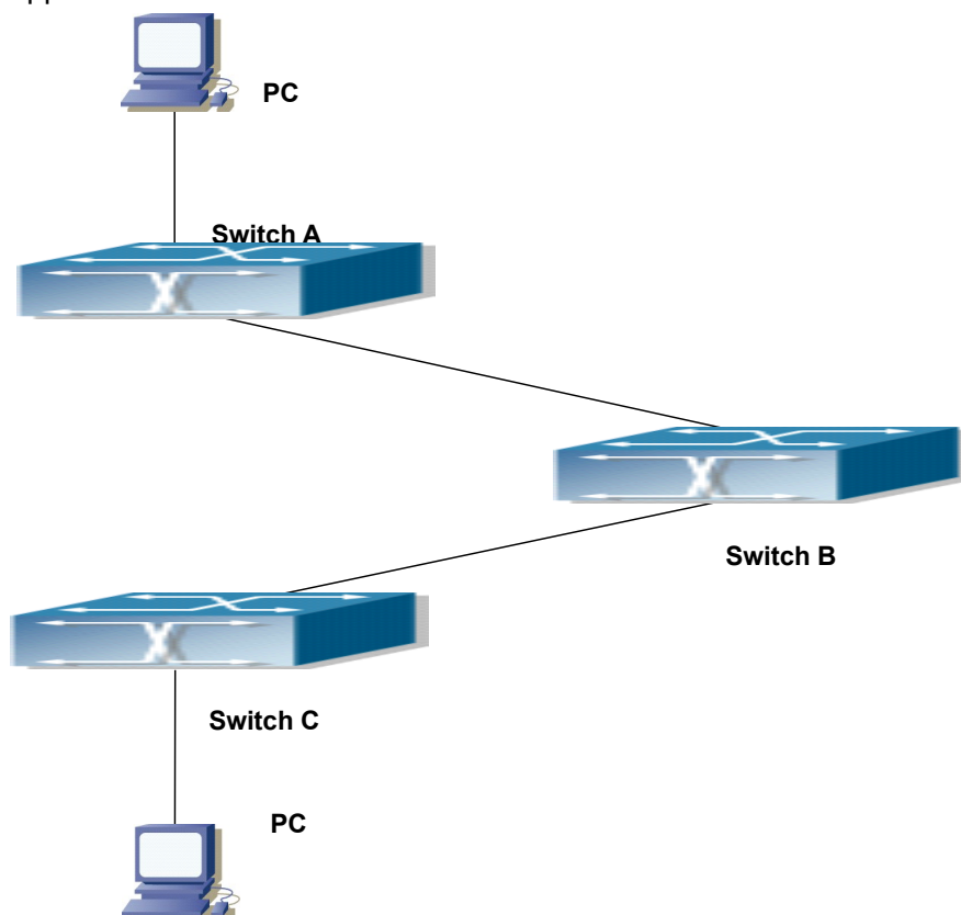
Fig 1-11 Typical GVRP Application Topology
